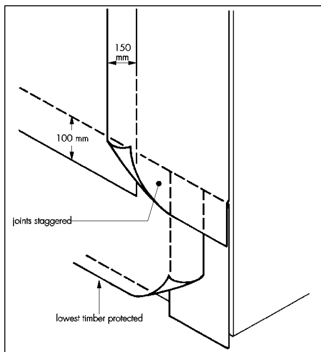
Figure 1 Membrane installation
